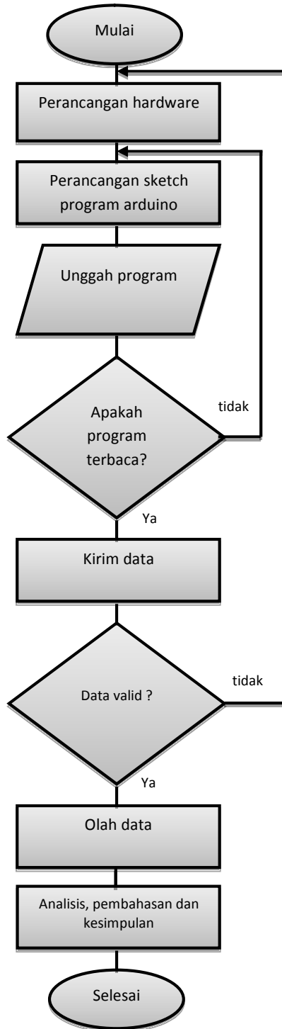
Gambar 2-1. Flowchart penelitian
