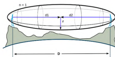
Gambar 2-1. Ilustrasi fresnel zone
